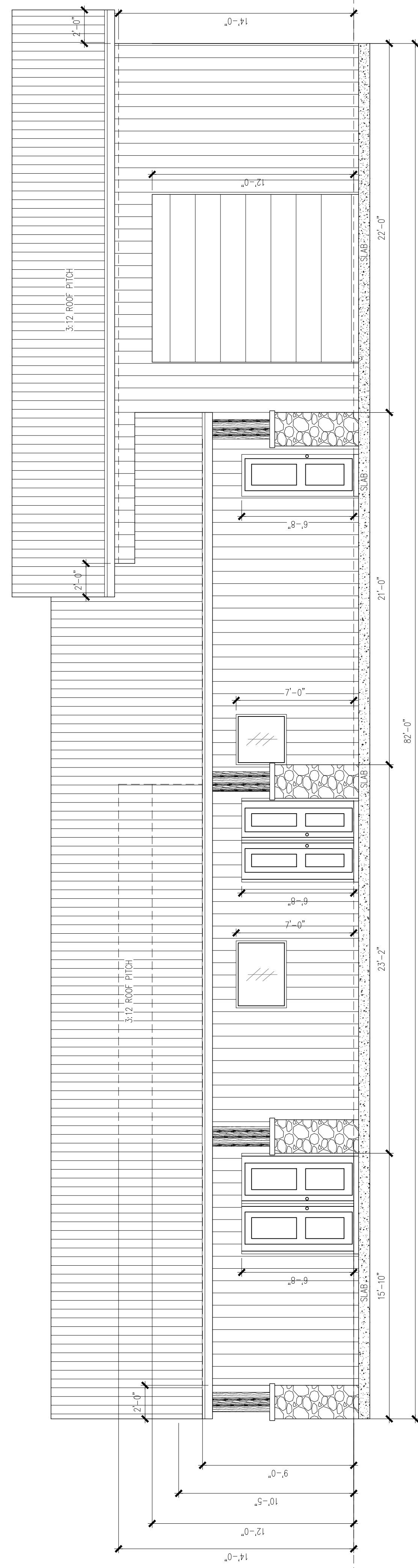
FRONT ELEVATION SCALE: 1/4"=1'-0"
